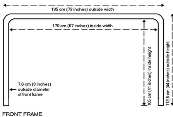
FRONT FRAME
