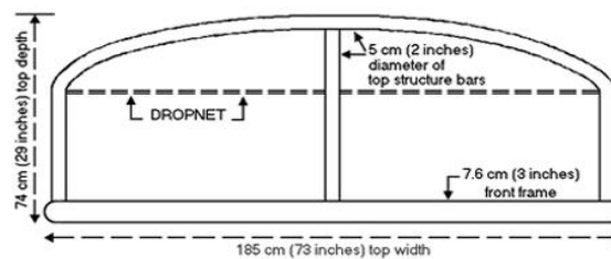
UPPER STRUCTURE
