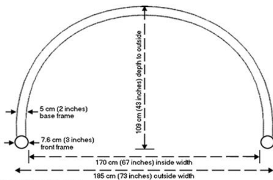
BASE STRUCTURE
